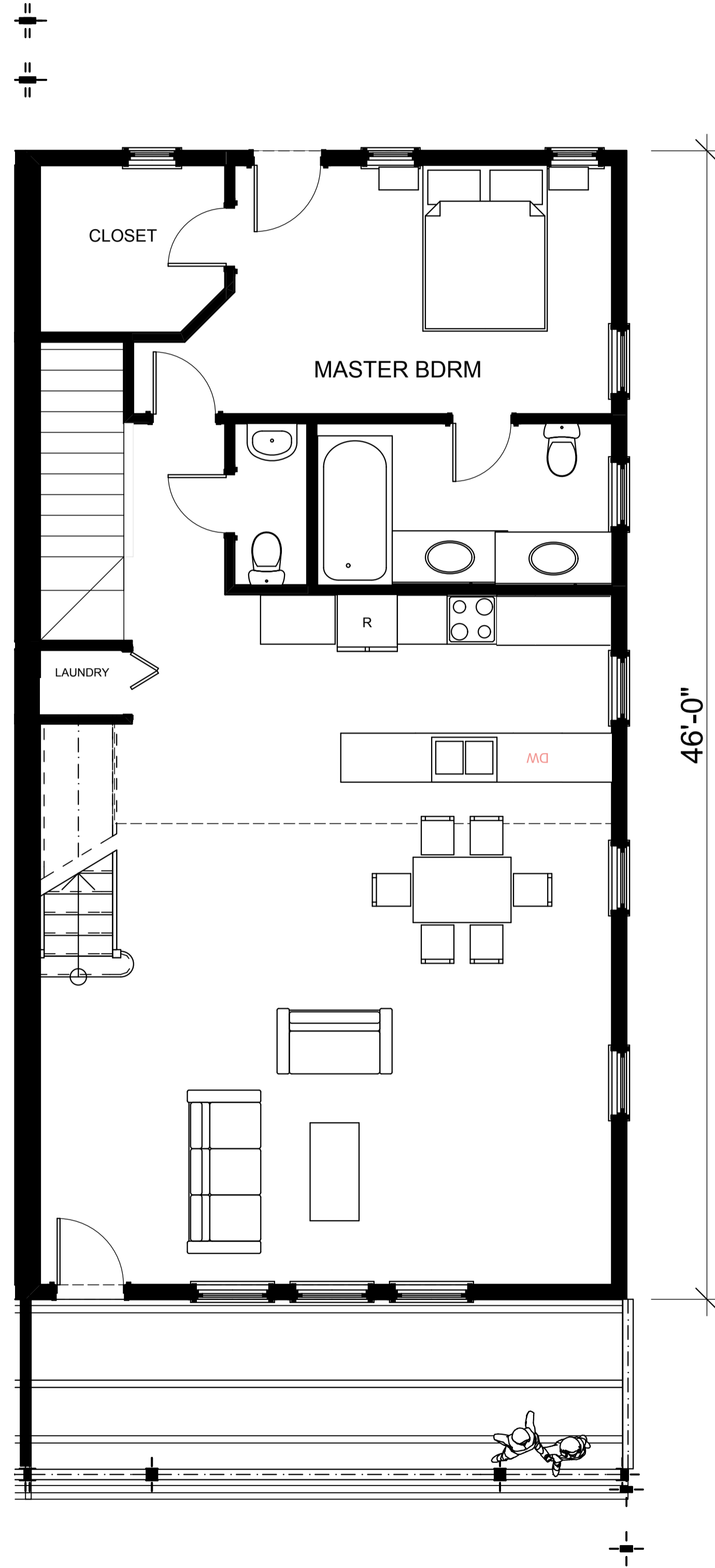
1 2nd FLOOR
